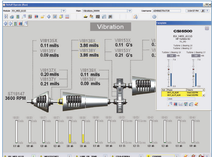
CSI 6500 faceplate and dynamos are included in DeltaV software. Dynamos allow users to drag and drop bargraphs and number elements on the screen to create graphics in no time — attach dynamo to the data point and your done.
